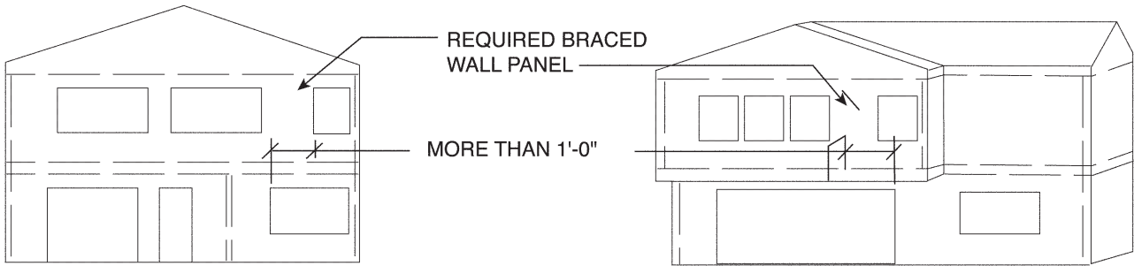
EXTERIOR ELEVATION
